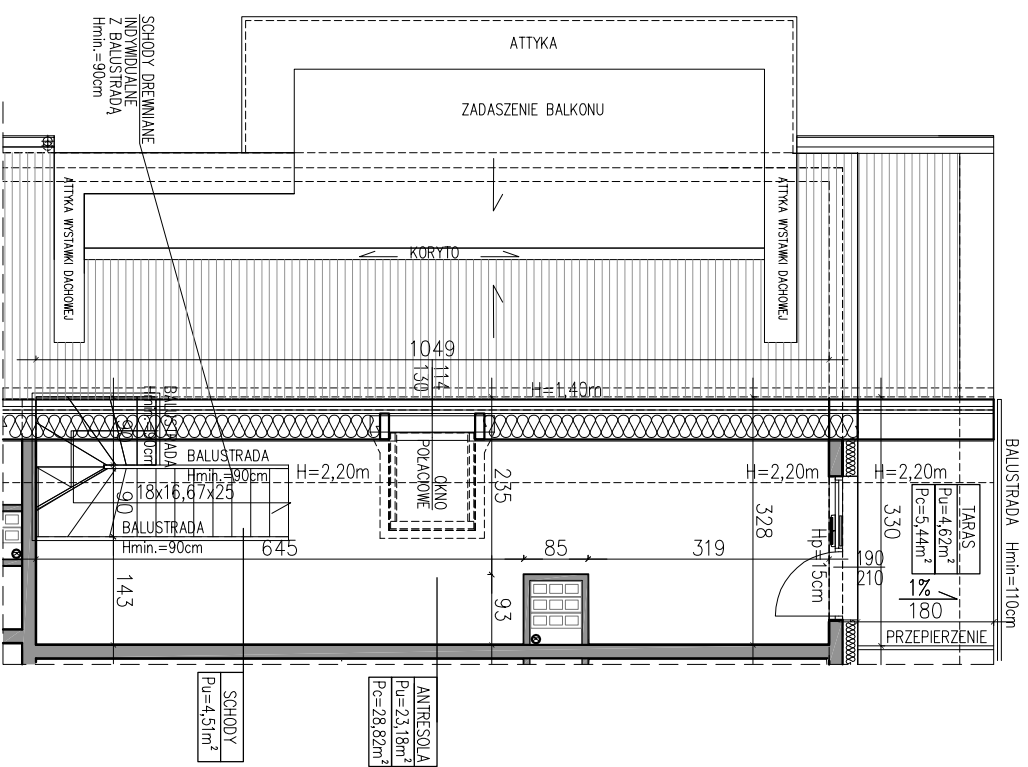
ANTRESOLA
